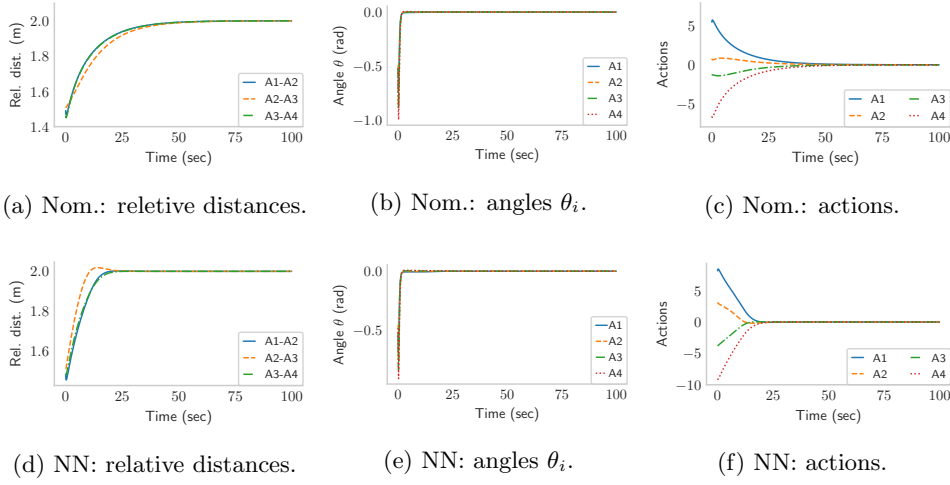
Fig. 5: State and action trajectories in a typical contral task, where the nominal controller (Nom) and the RL agents achieve costs of 58.3 and 41.0, respectively.
