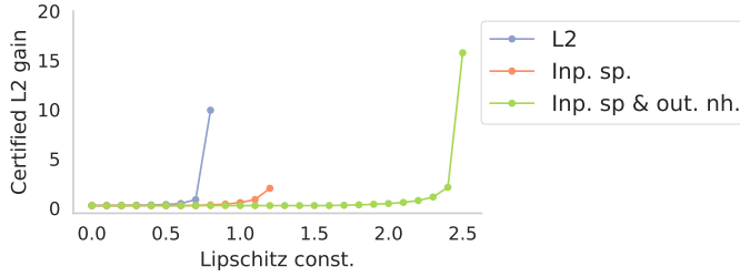
Fig. 3: Stability-certified Lipschitz constants obtained by the standard L_2 bound (L2) in (3.3) and the method proposed in Lemma 3.2, which considers input sparsity (inp. sp.) and output non-homogeneity (out. nh.).
