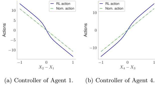
Fig. 6: Demonstration of control outputs for the nominal action and RL agents.
