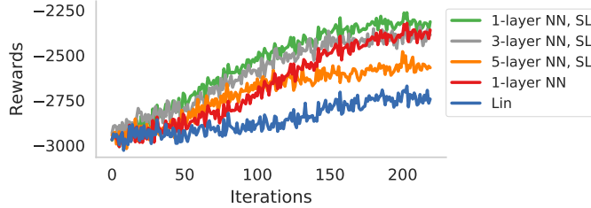
Fig. 4: Learning performance of different control structures (1-layer neural network, 5-layer neural network, and linear controller). By the inclusion of a smoothness loss (SL) in the learning objective (2.8), the exploration becomes more effective.
