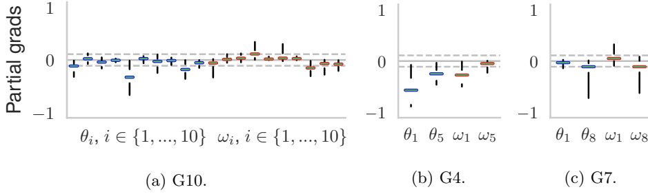
Fig. 9: Box plots of partial gradients of individual generators (G10, G4, G7) with respect to local information. Grey dashed lines indicate \pm 0.1 .
