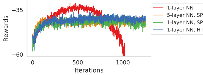
Fig. 11: Long-term performance of RL for agents with regulated gradients by soft penalty (SP), which adaptively adjusts the coefficients \omega_2 in (2.8), and hard thresholding (HT), which shrinks the network last layer to satisfy the gradient bounds. The RL agents without regulating the gradients exhibit “dangerous” behaviors in the long run.
