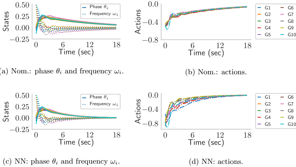
Fig. 10: State and action trajectories of the nominal and neural network controllers for power system frequency regulation, with costs of 50.8 and 23.9, respectively.
