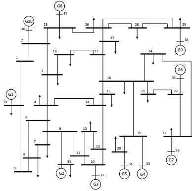
(b) IEEE 39-bus system.
