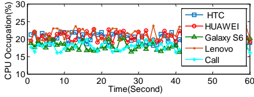
Figure 22: CPU utilization.
