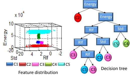
Figure 10: RSSI feature distribution and its decision tree ( C1 to C5 denotes the five RSSI profiles in Figure 9).
