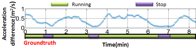
Figure 5: Acceleration trace of a train during a metro trip.
