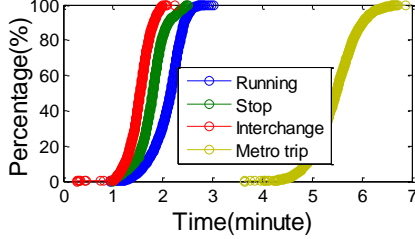
Figure 18: Accumulate error time.
